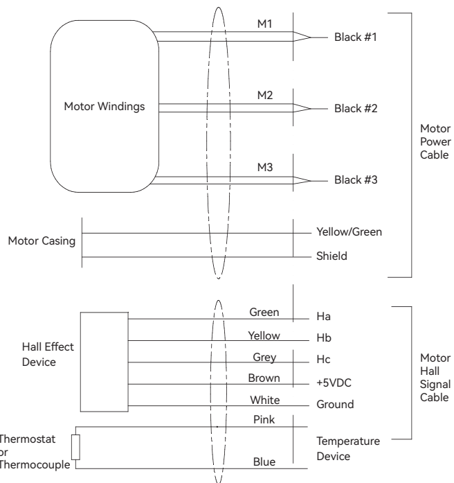
Cable Connection Information (600Vdc)
