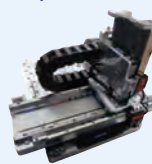
XYZ stage for mobile phone parts assembly
