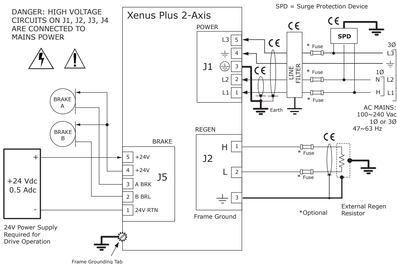
Power, Regen & Brake Connections Diagram
