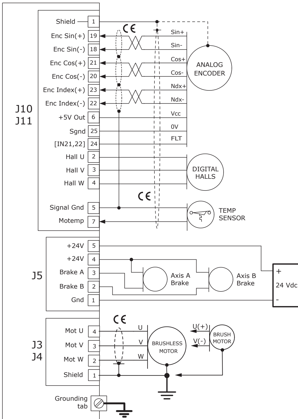
Analog Incremental Encoders Motor Connections Diagram
