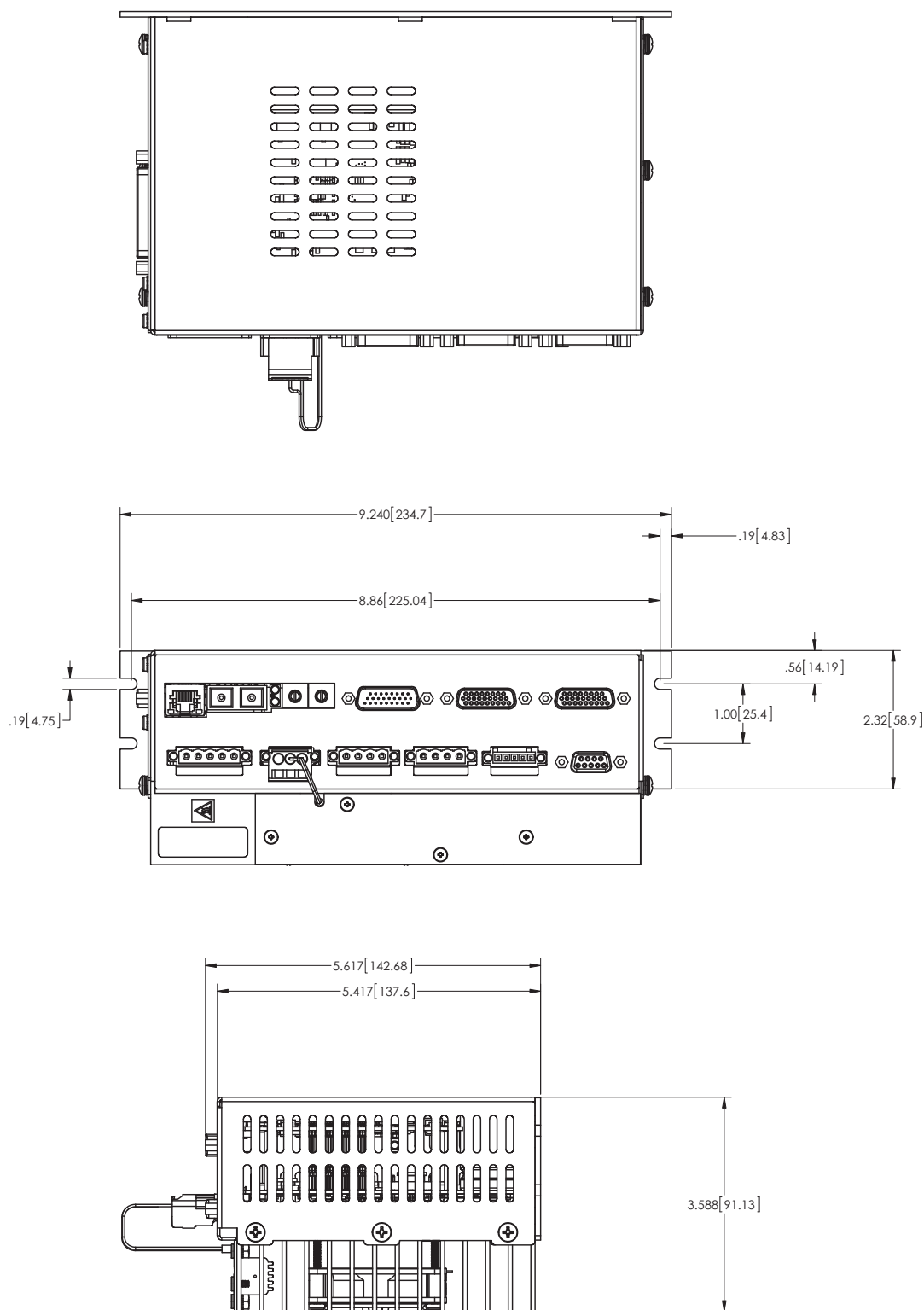
XM2 Dimensions Diagram
