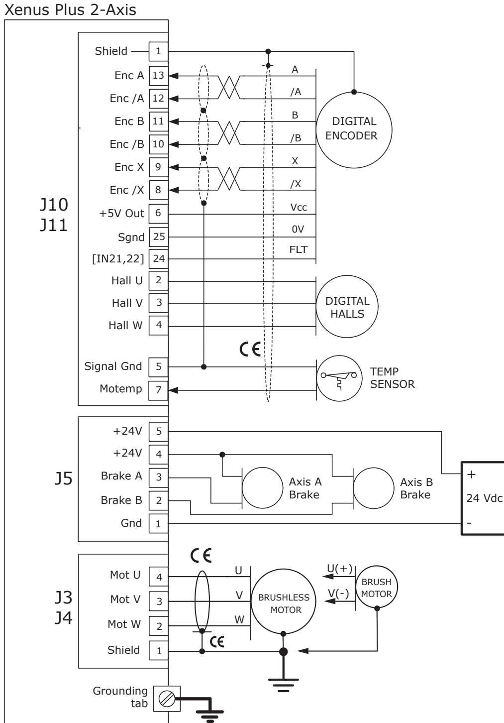
Digital Incremental Encoders Motor Connections Diagram
