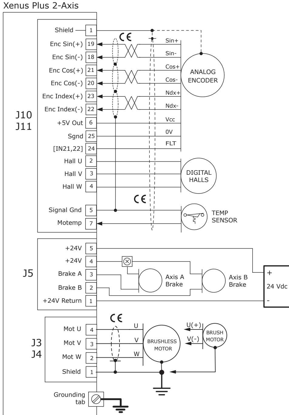
Analog Incremental Encoders Motor Connections Diagram
