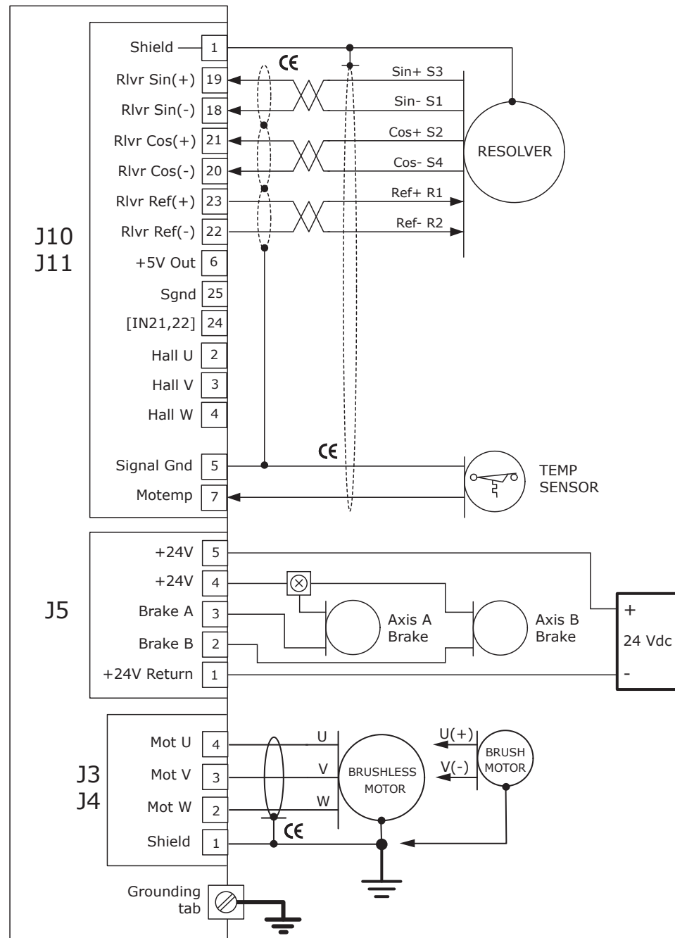
Resolvers Motor Connections Diagram
