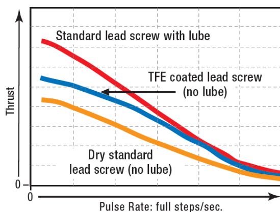
Lead Screw Comparison: FORCE vs. PULSE RATE – L/R Drive – 100% Duty Cycle
