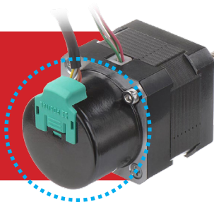
Size 17: 43 mm (1.7-in) Hybrid Linear Actuator (1.8° Step Angle)
