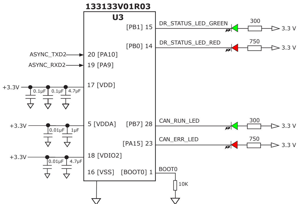
NPS-Z Switches & LEDs Diagram
