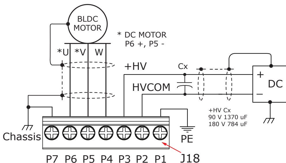
Motor Connections Diagram
