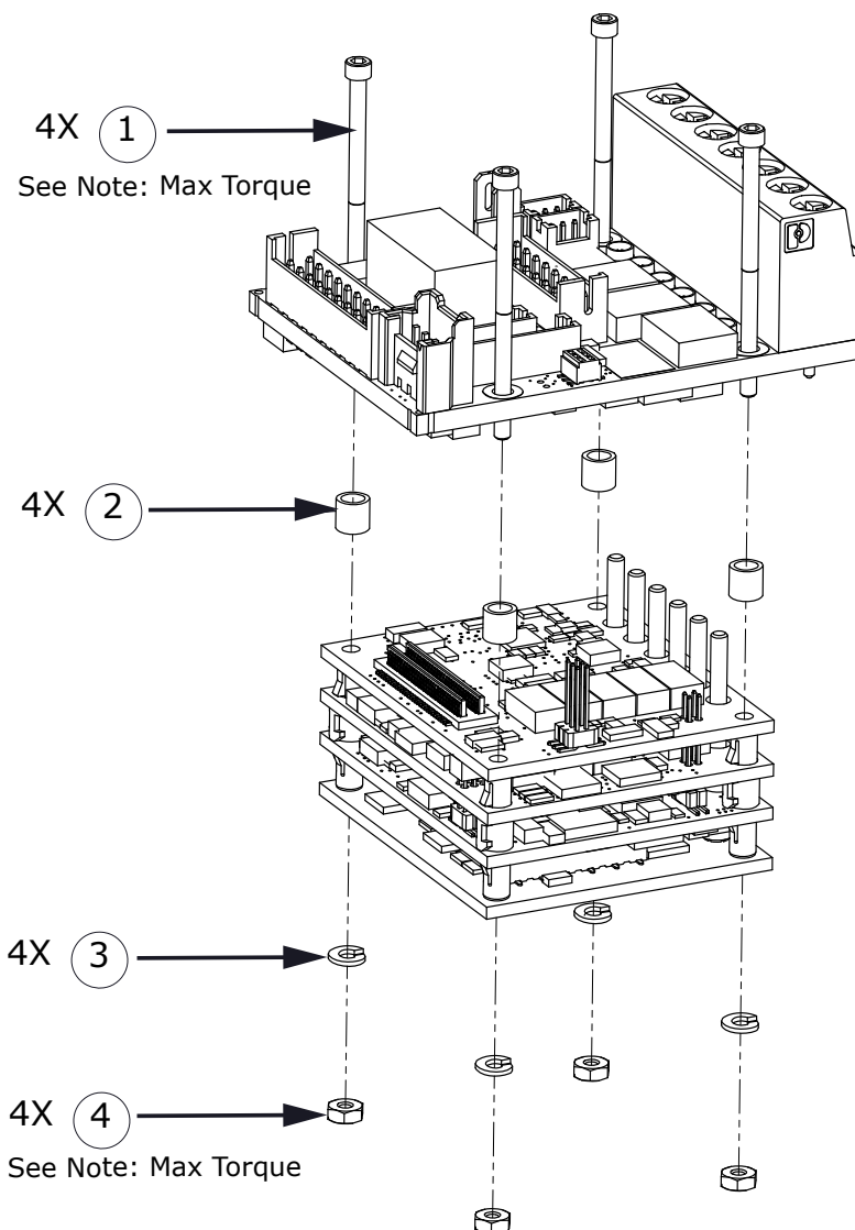
NPS-Z Components Diagram
