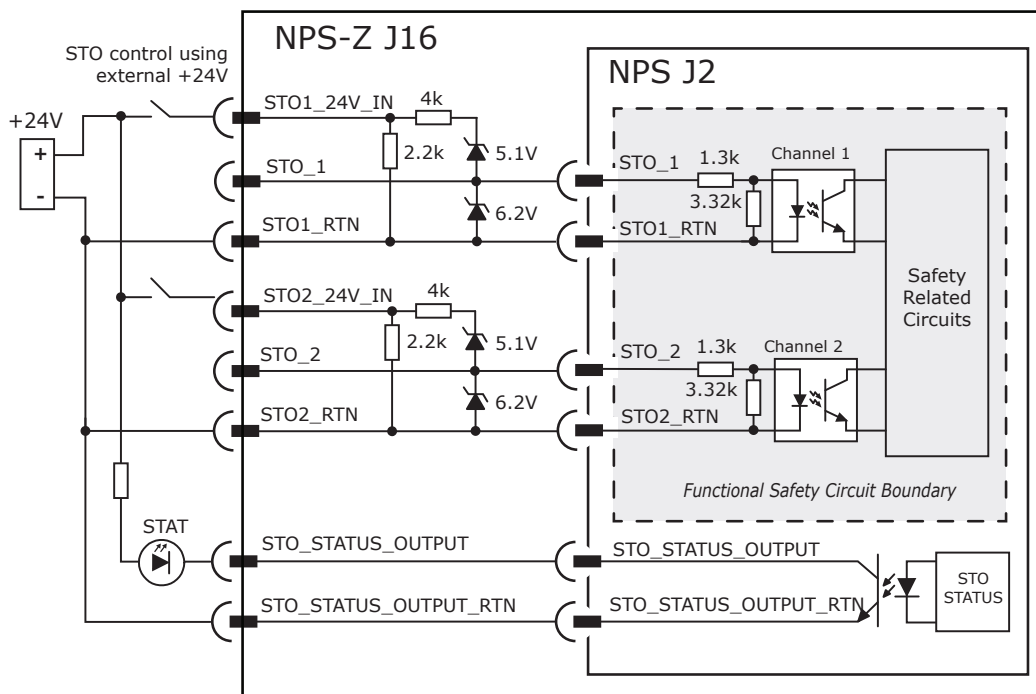
NPS-Z J16 (STO) Diagram
