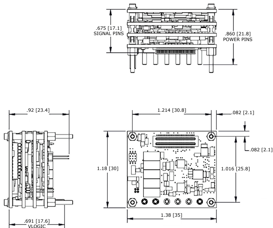
NPS Diagram (dimensions are in inches [mm])
