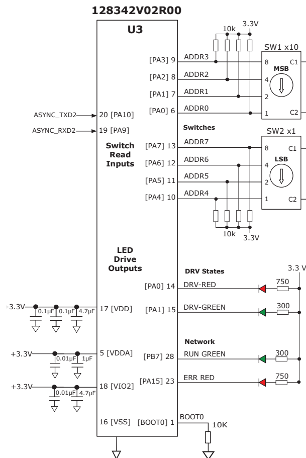
NPS-D Switches & LEDS Diagram
