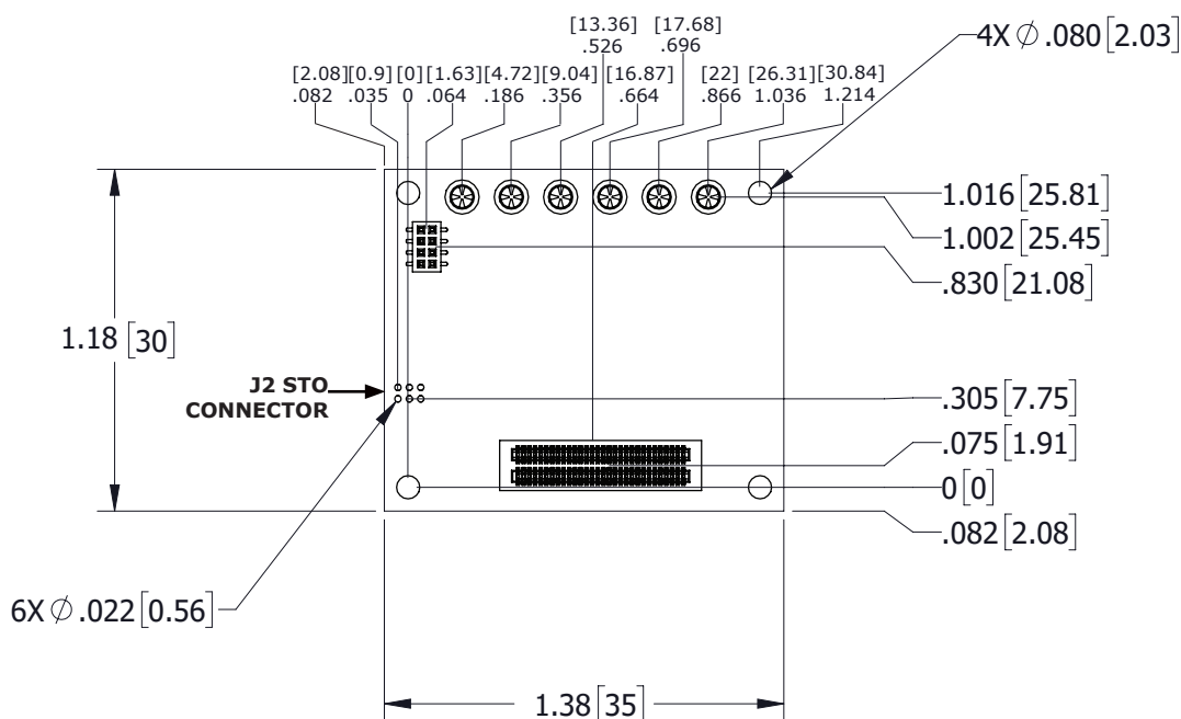
User Mounting Board Dimensions (Topside View) Diagram
