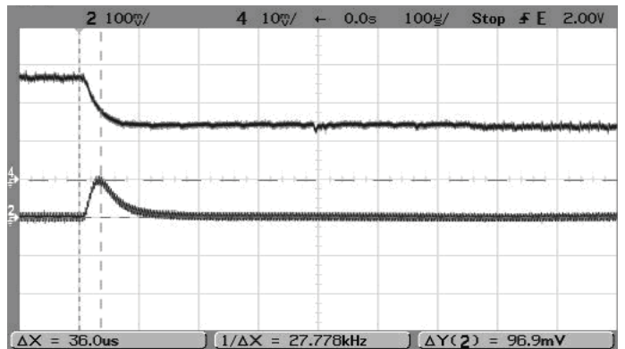
Step Load Transient Response (Vin=5V, Vout=2.5V, Cload=0, Iout=5A to 2.5A) Trace 2=Vout, 100 mV/div. Trace 4=Iout, 2A/div.
