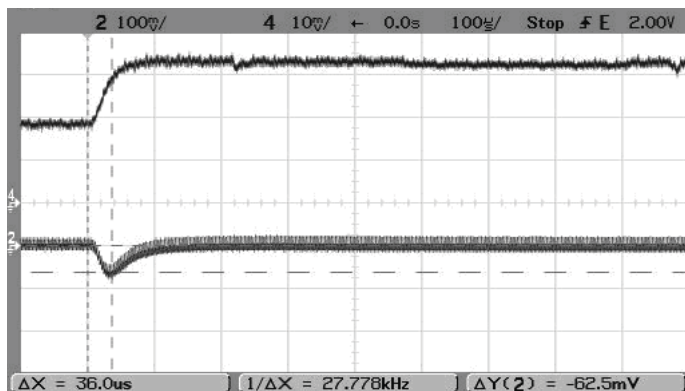
Step Load Transient Response (Vin=5V, Vout=1.8V, Load=0, Iout=1.5A to 3A) Trace 2=Vout, 100 mV/div. Trace 4=Iout, 1A/div.
