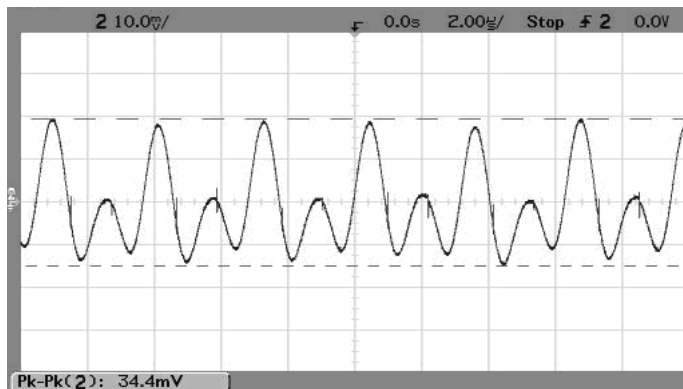
Output Ripple and Noise (Vin=5V, Vout=1.8V, Iout=3A, Load=0, ScopeBW=100MHz)
