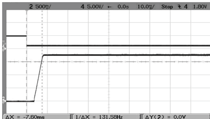
On/Off Enable Startup (Vin=5.5V, Vout=1.8V, Iout=3A, Load=0) Trace 4=Enable, Trace 2=Vout
