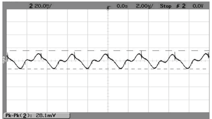
Output Ripple and Noise (Vin=5V, Vout=2.5V, Iout=5A, Cload=0, ScopeBW=100MHz)
