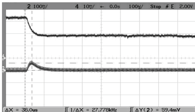
Step Load Transient Response (Vin=5V, Vout=1.8V, Load=0, Iout=3A to 1.5A) Trace 2=Vout, 100 mV/div. Trace 4=Iout, 1A/div.
