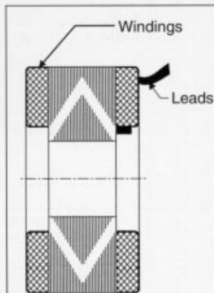
Figure 2. Frameless armature assembly
