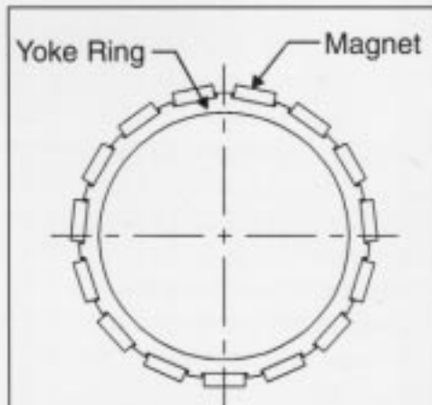
Figure 3. Basic configuration for a field assembly.
