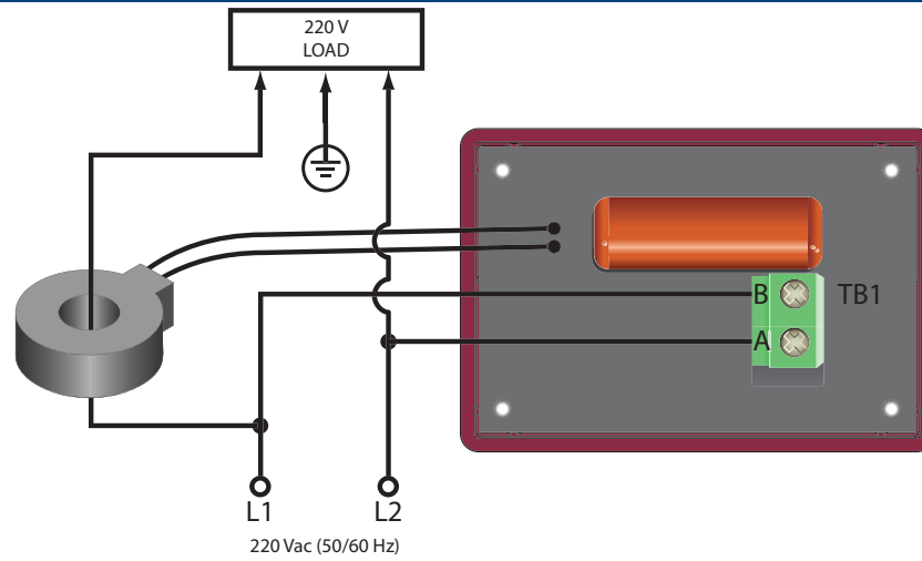
Figure 2. Wiring diagram for 220/240V systems with no neutral
