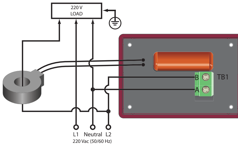
Figure 4. Wiring diagram for 220/240V systems with neutral (monitoring phase L2)
