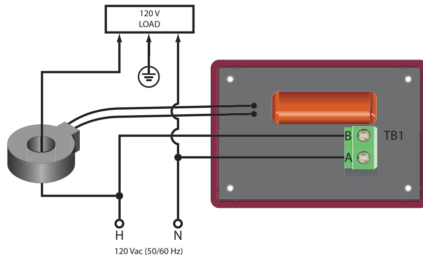
Figure 1. Wiring diagram for 110/120V single phase systems
