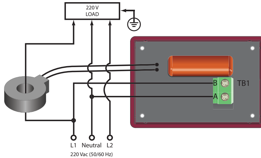
Figure 3. Wiring diagram for 220/240V systems with neutral (monitoring phase L1)
