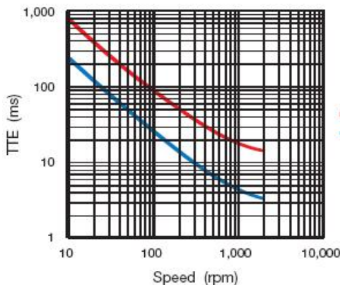
EC75, EC75LL Time to Engage vs. Speed
