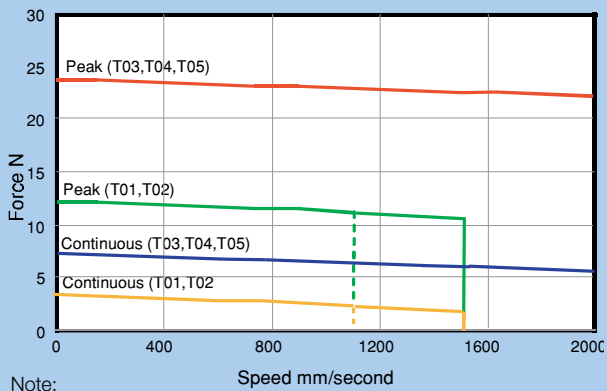
Force - Speed
